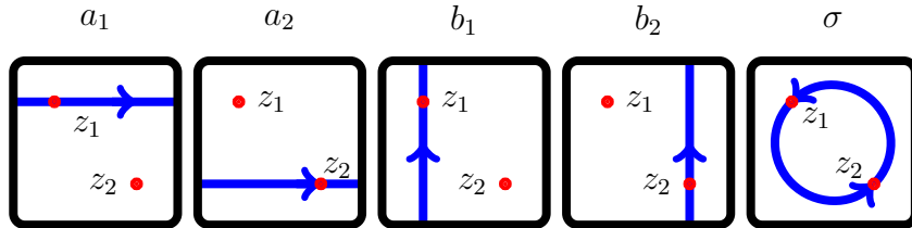
FIGURE 2.1. Generators of the braid group \mathbf{B}_2(\mathbf{T}^2) .
