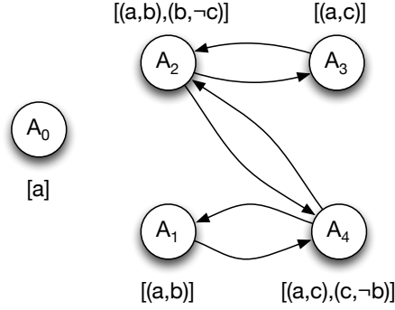
Fig. 8. Argumentation framework constructed from a preordered hierarchical abstract normative system.
