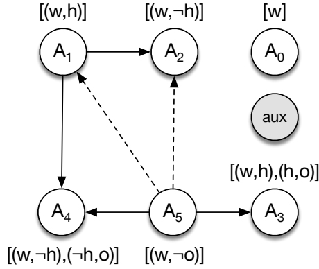
Fig. 6. Argumentation framework expanded by an auxiliary argument and two auxiliary defeats (denoted using dashed lines).
