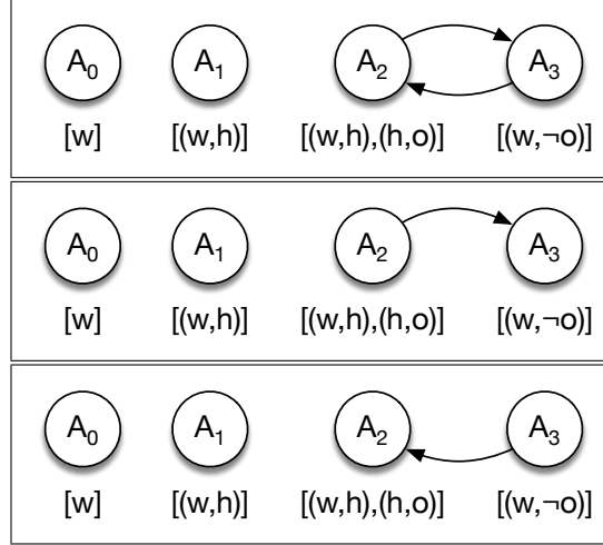
Fig. 2. Top: the argumentation framework obtained from the order puzzle hierarchical normative system with the four arguments and attacks between them visualized as directed arrows. Middle: the argumentation framework obtained when last link is applied. Bottom: the argumentation framework obtained when weakest link is applied.
