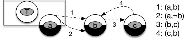
Fig. 3. The hierarchical abstract normative system of Example 2.7 containing the two Reduction extensions \{b, c\} and \{\neg b\} .
