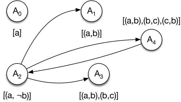
Fig. 4. The argumentation framework obtained for the hierarchical abstract normative system of Figure 3.
