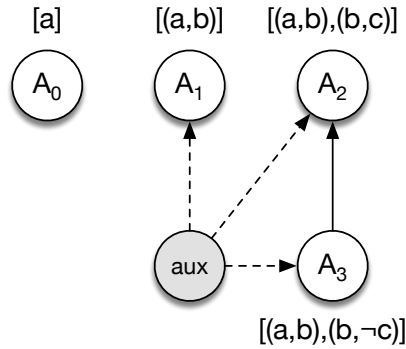
Fig. 7. Argumentation framework expanded by an auxiliary argument and three auxiliary defeats (denoted using dashed lines).
