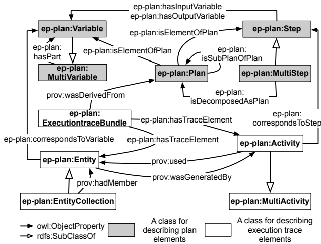
Figure 3: An overview of a subset of EP-Plan concepts for describing and linking plan specifications with their execution traces.
