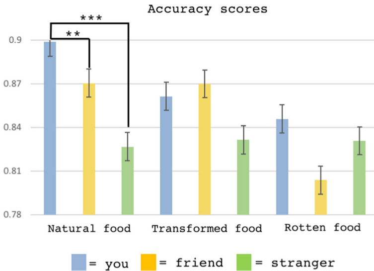
Fig. 3 Accuracy scores
