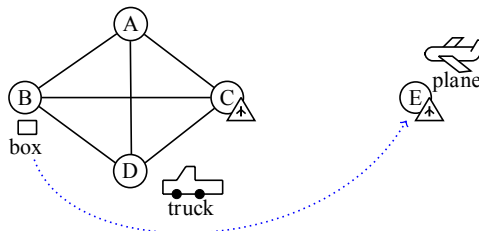
Figure 3: LOGISTICS problem example with goal (at BOX AIRPORT-E).
