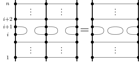
(a) The relation U_i^2 = aU_i .
