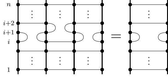
(b) The relation U_i U_{i+1} U_i = U_i .
