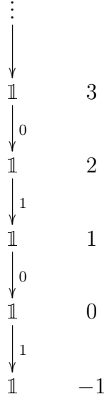
FIGURE 5. The complex \mathbb{1} \otimes C(m)
