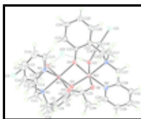
Fig. 1. The molecular structure of the ionic components comprising (I) showing the atom-labelling scheme and displacement ellipsoids at the 50% probability level. The O–H \cdots Cl hydrogen bonds are shown as black dashed lines.
