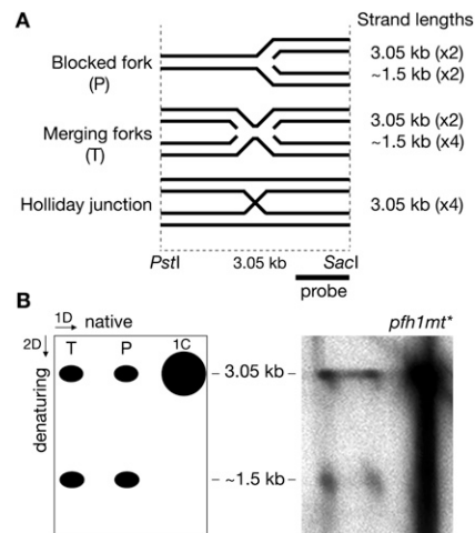
Figure 5. X-shaped DNA molecules that accumulate at RTS1 in a pfh1mt* mutant are opposing replication forks in the final stages of merging. (A) Schematic showing the expected single-strand lengths of different types of junction positioned at RTS1 in the PstI–SacI fragment described in Figure 3. (B) Neutral-alkaline 2D gel analysis of replication intermediates in the PstI–SacI fragment shown in Figure 3A from pfh1mt* cells. The schematic shows the position of linear duplex (1C), paused replication fork (P), and X-shaped termination signal (T).
