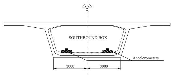
Figure 3. Location of accelerometers inside bridge girder
