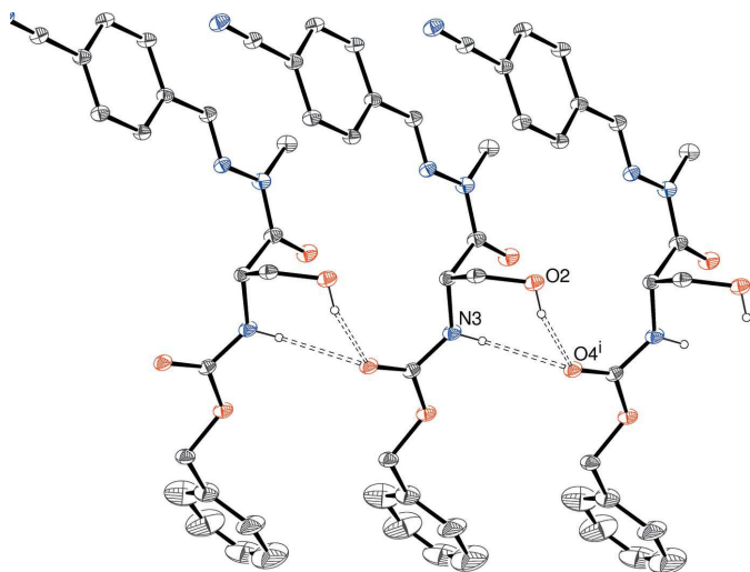
Figure 4 Fragment of a [100] hydrogen-bonded chain in the crystal of (I). Symmetry code: (i) 1 + x, y, z . All C-bound H atoms are omitted for clarity.
