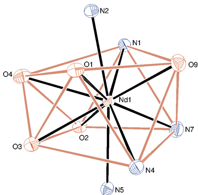
Figure 4 Detail of (II) showing the distorted bicapped square-antiprismatic \text{NdO}_5\text{N}_5 coordination polyhedron (contacts between the atoms forming the square antiprism indicated with tan lines). Displacement ellipsoids are shown at the 50% probability level.
