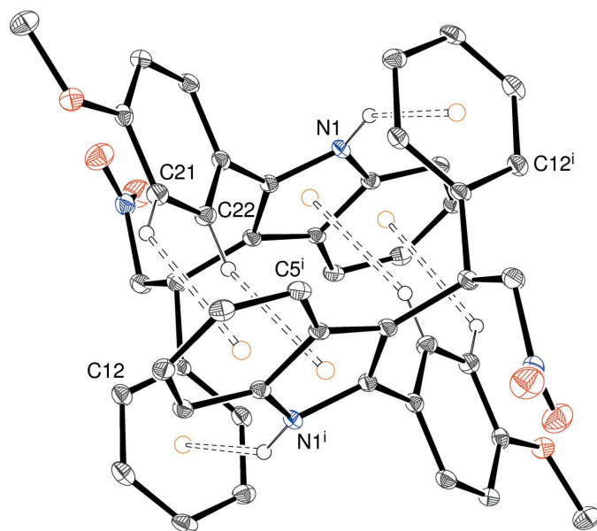
Figure 6 An inversion dimer of N1 molecules in the crystal of (II) linked by pairs of N–H··· \pi and C–H··· \pi interactions (double-dashed lines). [Symmetry code: (i) 1 - x, -y, -z .] The N3 molecules associate into similar dimers. The orange circles indicate ring centroids.
