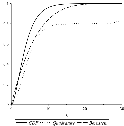
Fig. 4. [a, b] = [0, 30] .
