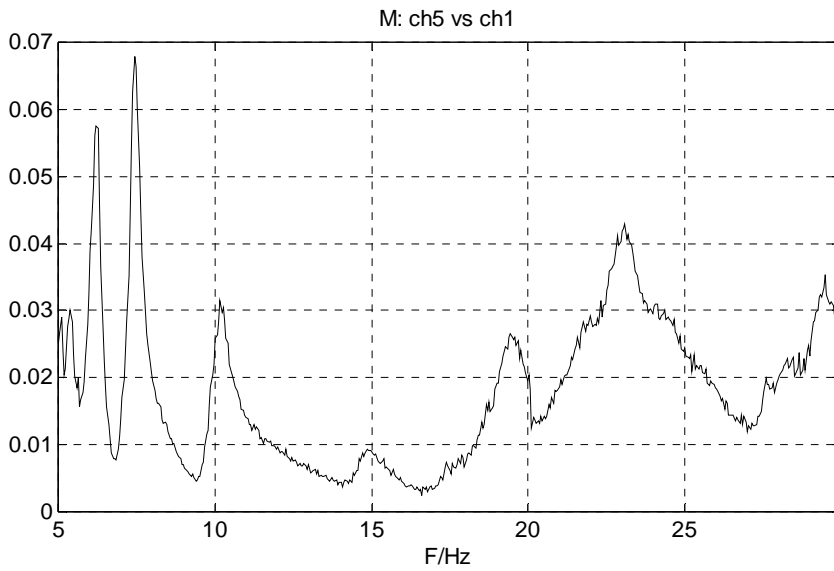
Figure 13 Pioneer Bridge FRF before and after upgrade showing increase in stiffness and damping capacity
