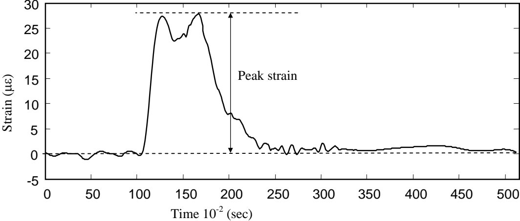
Figure 11: Typical strain record
