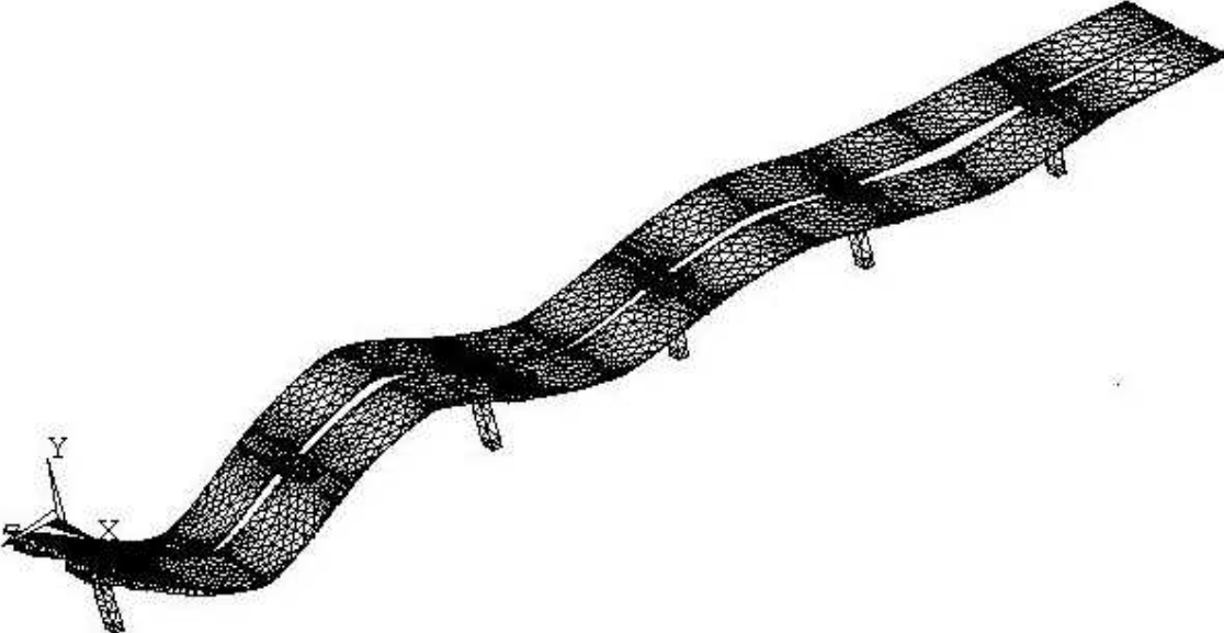
Figure 17 Extrusion of FE model to complete 'bridge'
