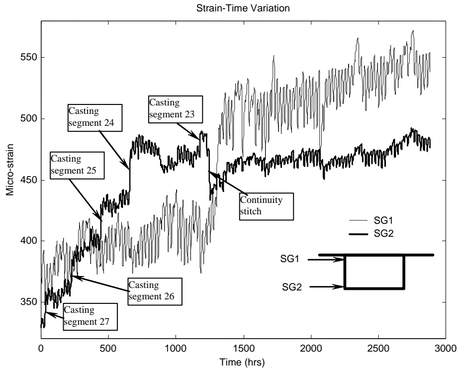
Figure 5 Strain variation in segment 31 during construction.
