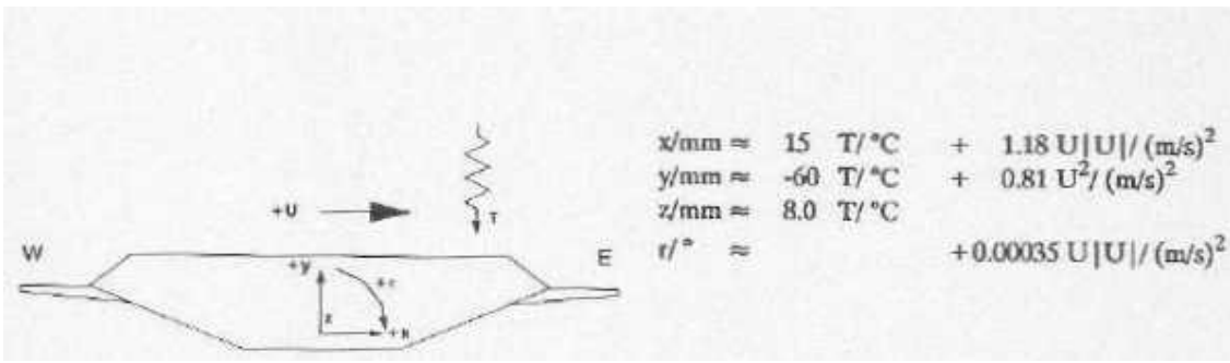
Figure 2 Correlations of external influences and structural responses
