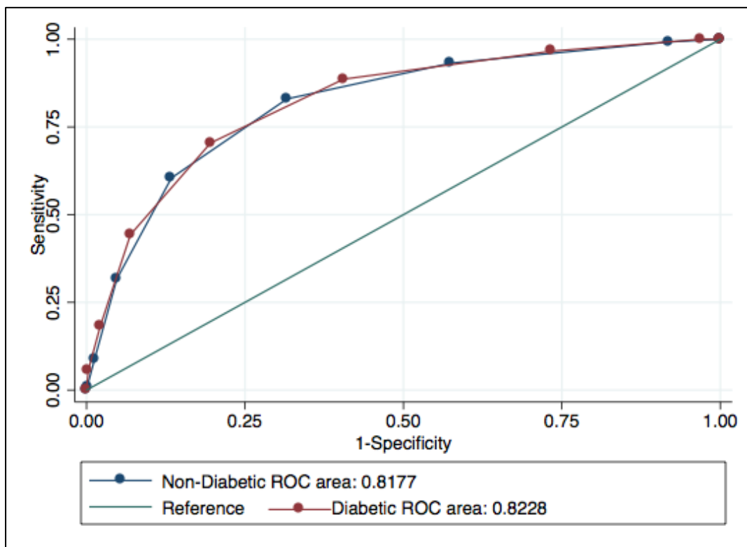
Figure 2f. Receiver Operating Characteristic curve differentiating 7-day mortality using SOAR with glucose score stratified by diabetes status before diagnosis
